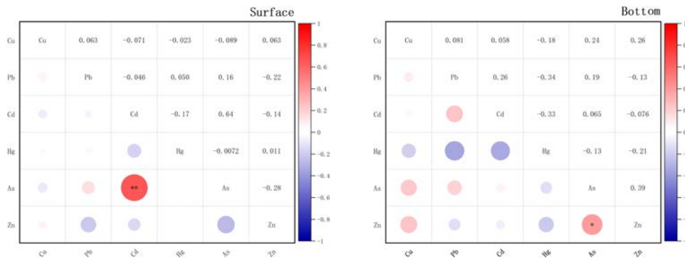
FIGURE 4 The correlation analysis of HMs in the seawater of Jieshi bay, respectively ( P < 0.05 , P < 0.1 ).
